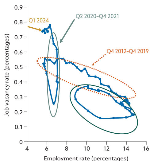
Chart 16 Beveridge curve
